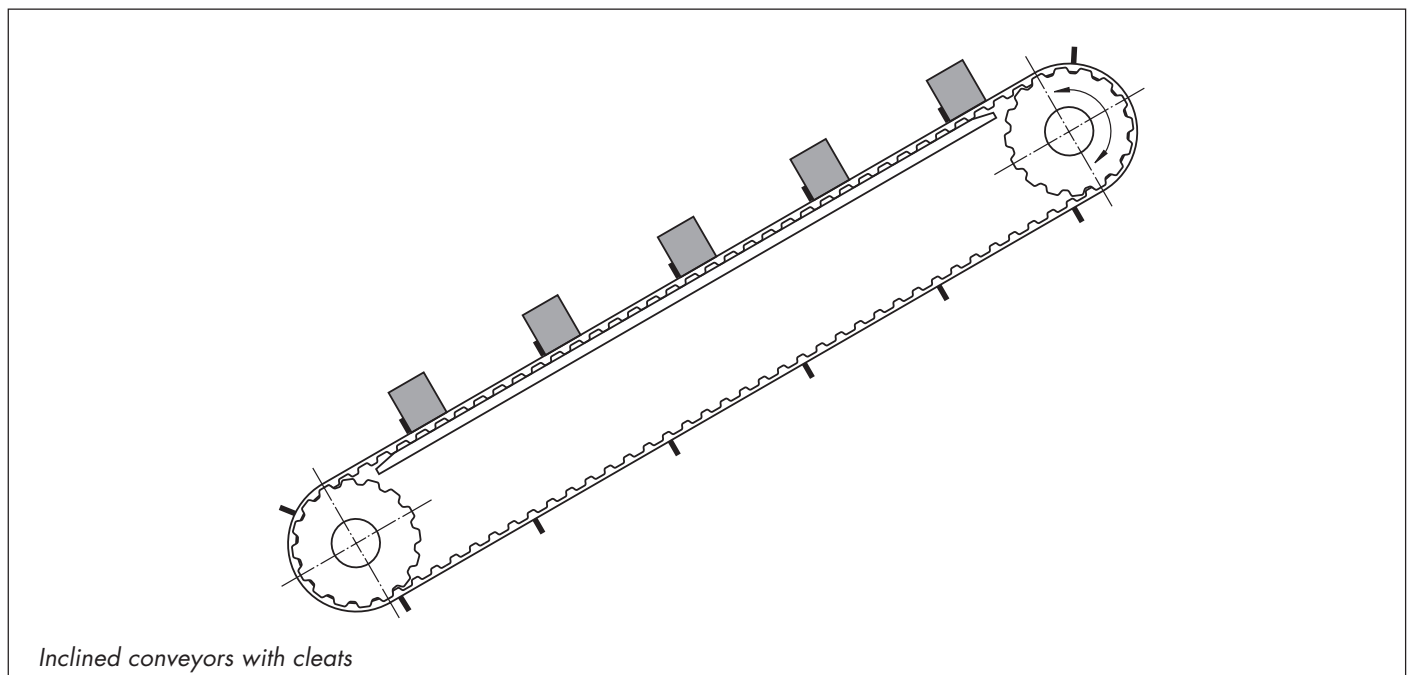
Fig. 1.4.3: Conveying
