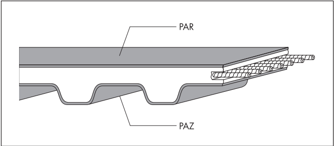
Fig. 1.6: Timing belt with fabric facing on both sides
