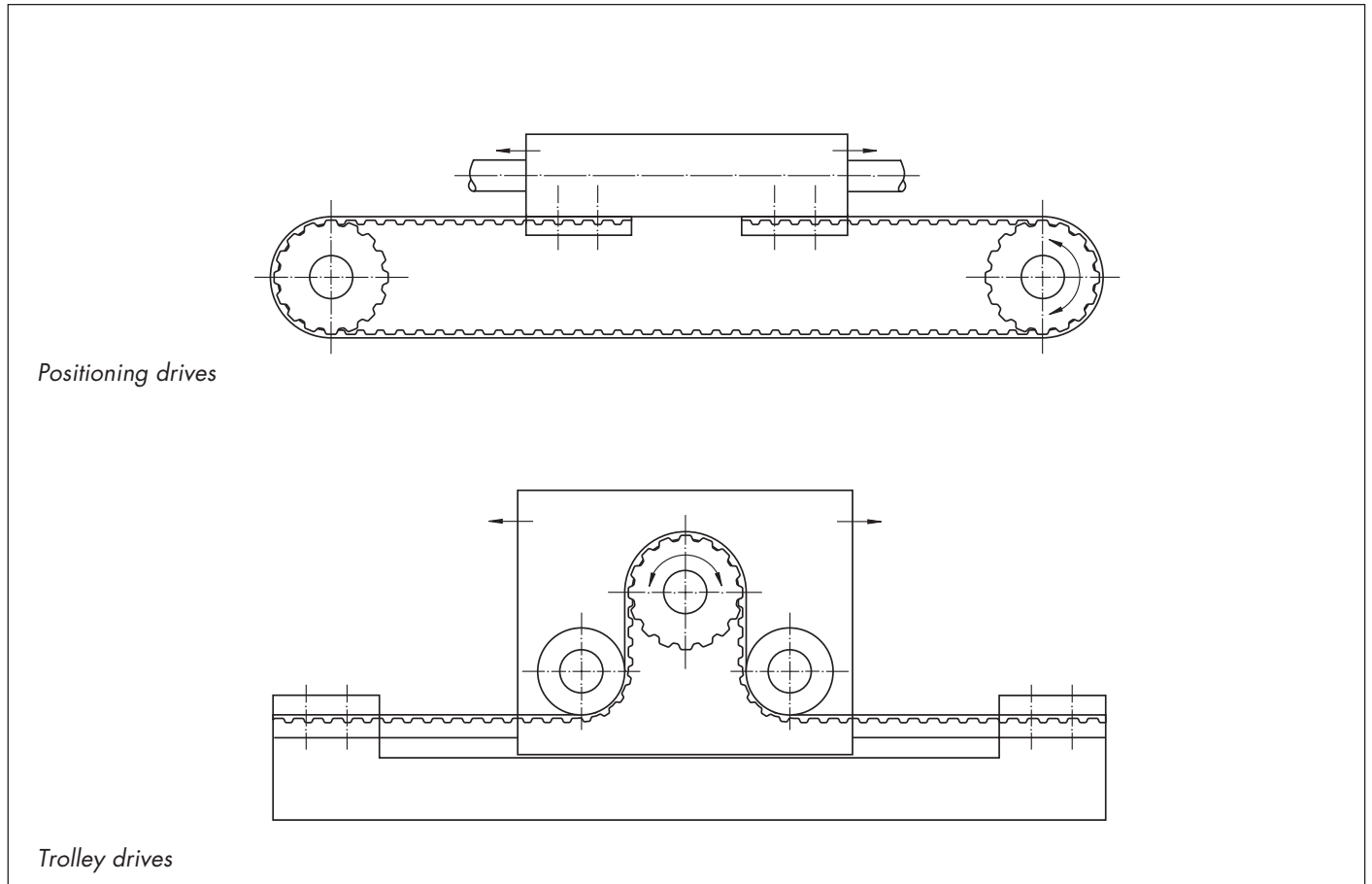
Fig. 1.4.2: Linear drives
