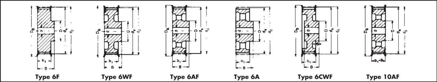
Type L – Pitch 9.525 mm for belt width 075
